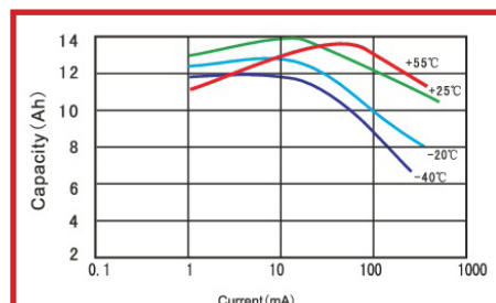
Capacity / Current (cutoff 2.0V)
