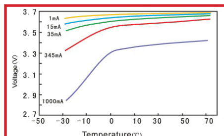
Volt/Temperature
